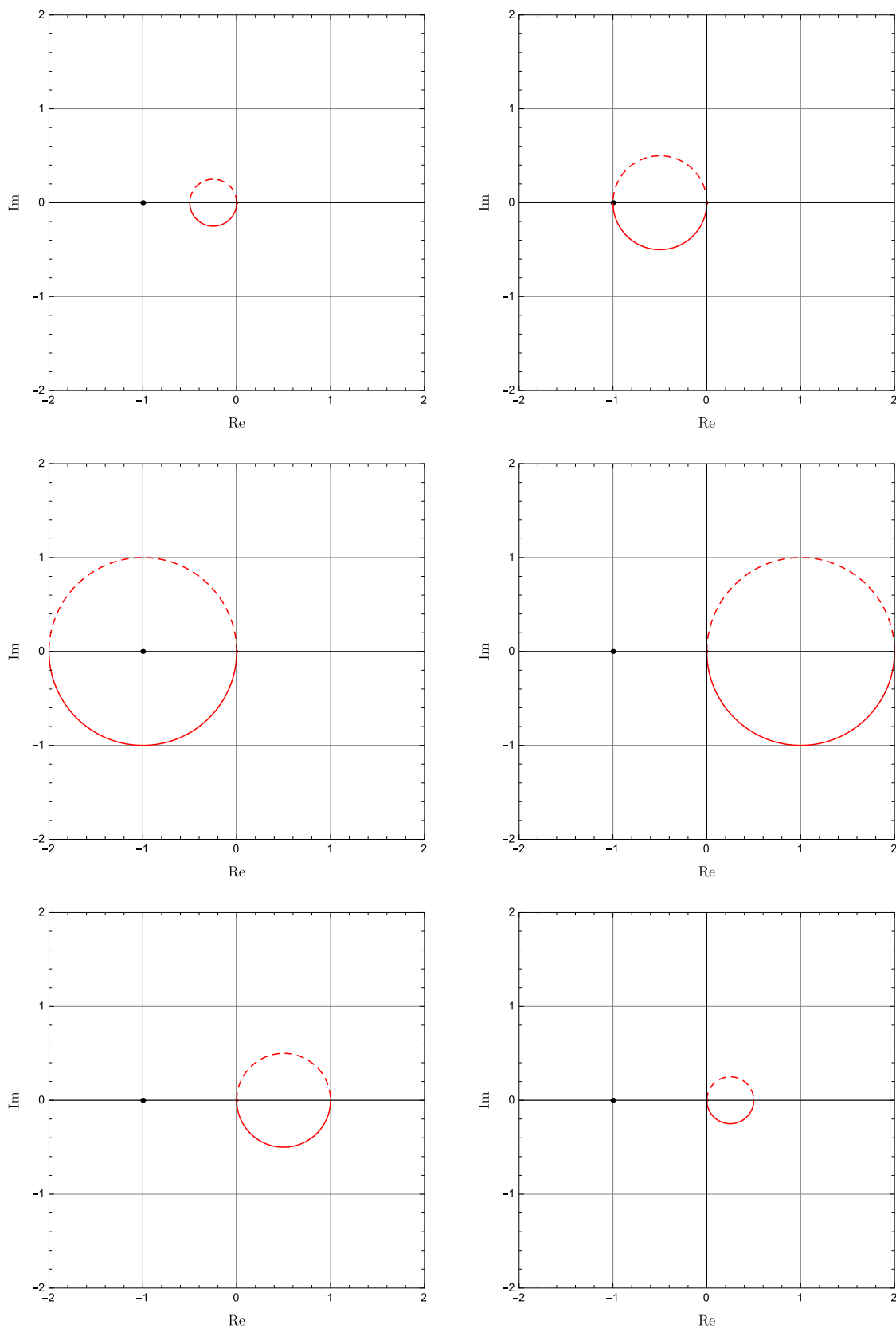
Figure 7.4 The (\infty, 0) -Nyquist contour for R_L(s) = \frac{1}{s+a} , a = -2 (top left), a = -1 (top right), a = -\frac{1}{2} (middle left), a = \frac{1}{2} (middle right), a = 1 (bottom left), and a = 2 (bottom right)
