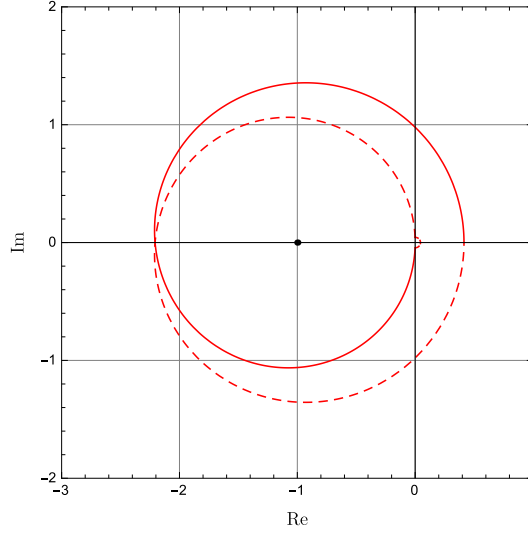
Figure 14.2 Nyquist plot for optimal state feedback with two unstable eigenvalues
