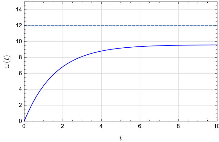
Figure 1.5 Open-loop response of DC motor with “actual” motor time-constant
