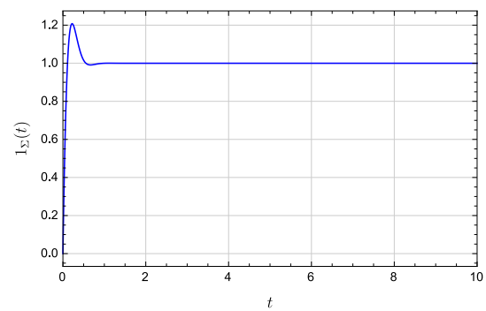
Step response 2
