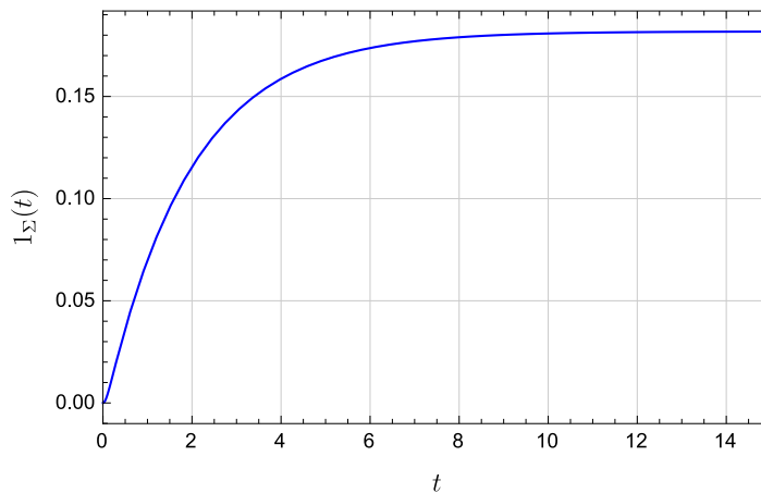
Figure 12.12 Step disturbance response of mass with lead compensator
