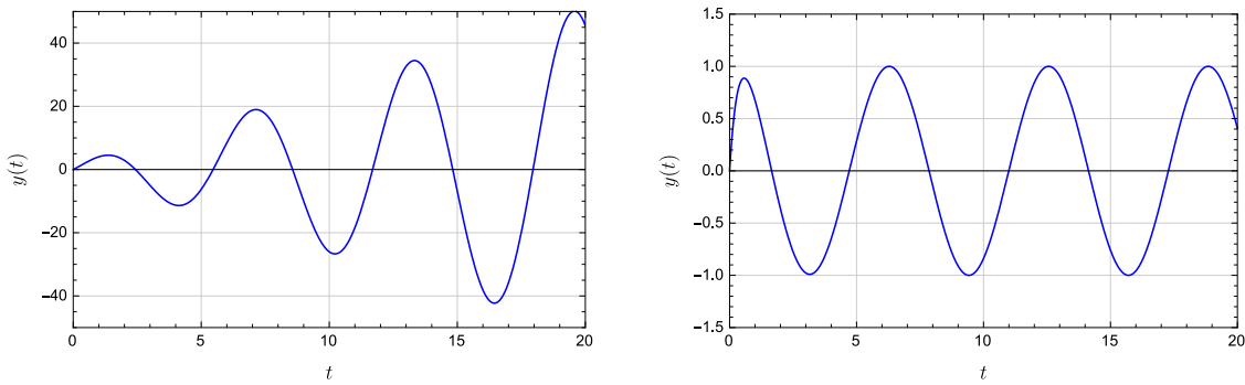
Figure 6.31 Output response for open-loop system (left) and closed-loop system (right) under static output feedback
