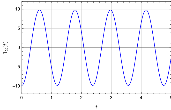
Figure 8.20 Response of falling mass to step disturbance with proportional control
