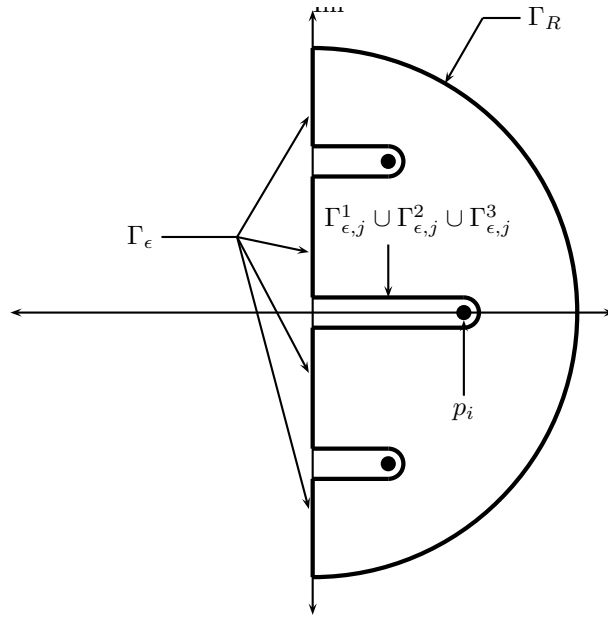
Figure 9.4 The contour for the Bode integral formulae
