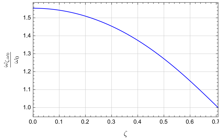
Figure 8.9 Dependence of bandwidth on \zeta for second-order systems
