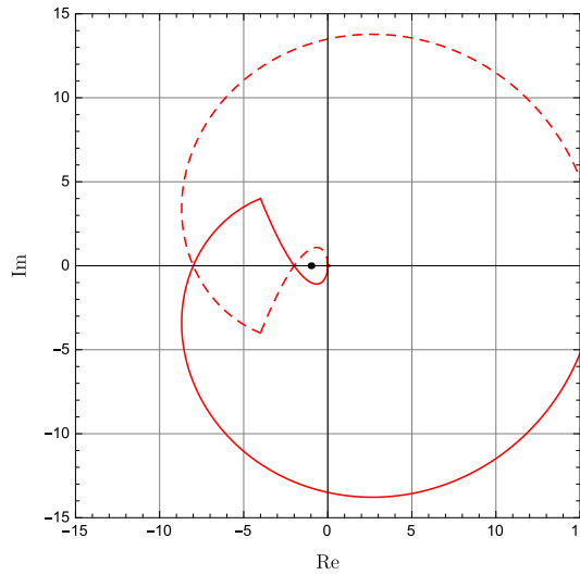
Figure 7.22 Nyquist plot for PID controller and nominal plant
