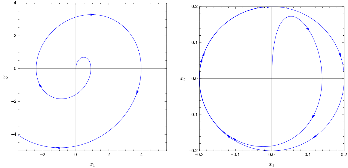
Figure 6.28 State response for open-loop system (left) and closed-loop system (right) under static state feedback
