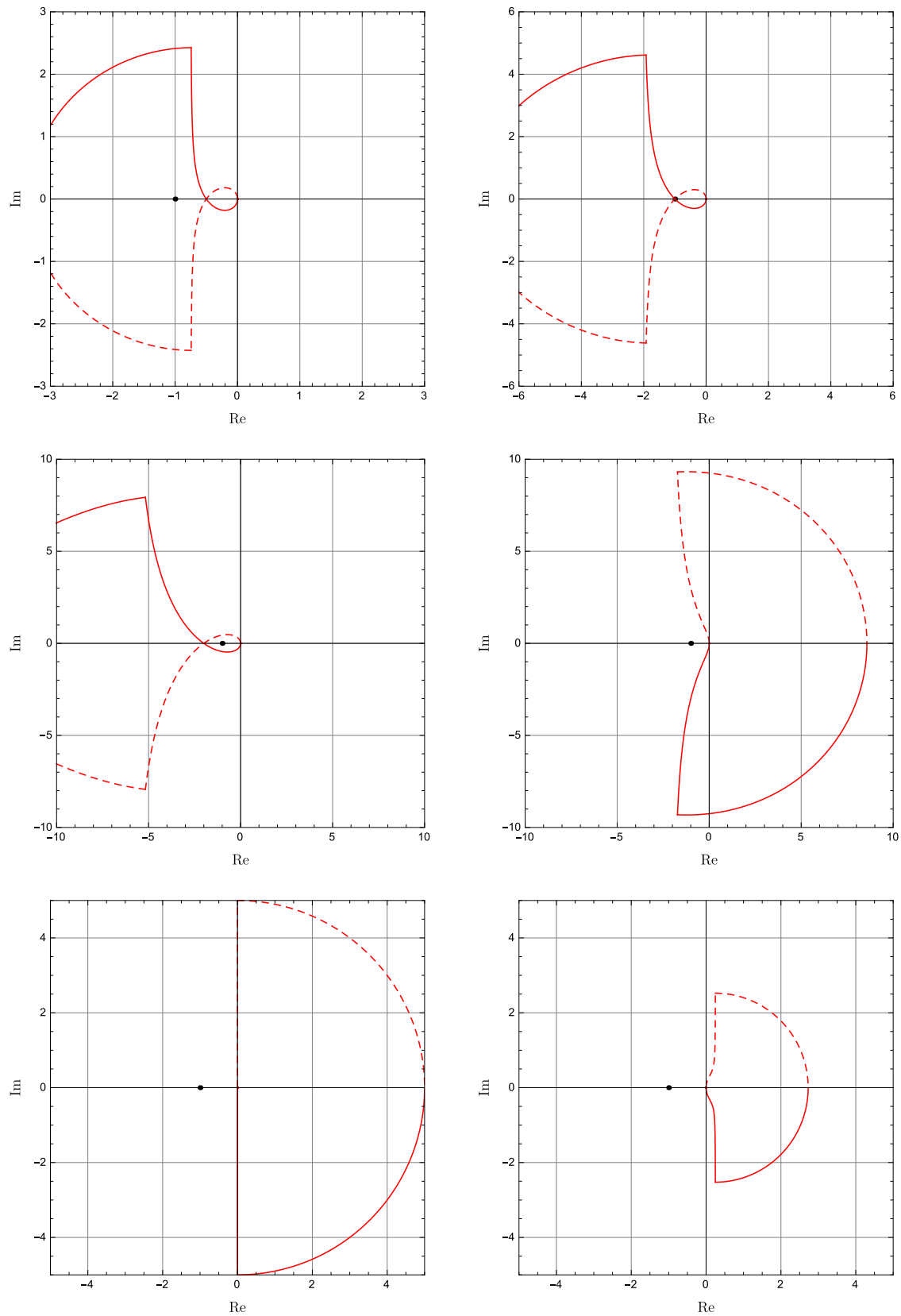
Figure 7.8 The (\infty, 0.2) -Nyquist contours for R_L(s) = \frac{s+1}{s(s+a)} , a = -2 (top left), a = -1 (top right), a = -\frac{1}{2} (middle left), a = \frac{1}{2} (middle right), a = 1 (bottom left), and a = 2 (bottom right)
