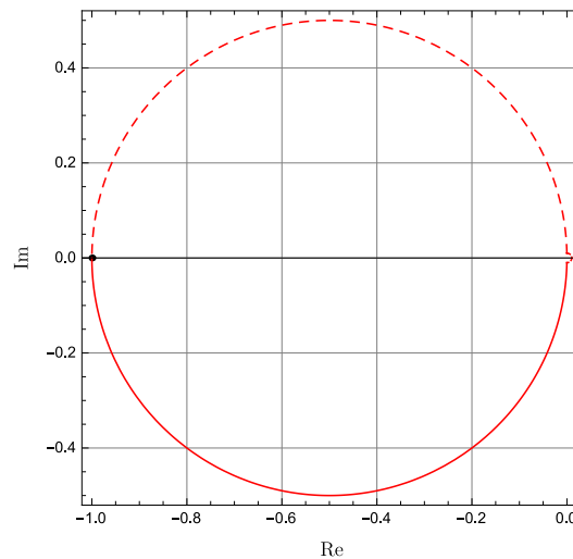
Figure 12.5 Stabilising an open-loop unstable system using the Nyquist criterion
