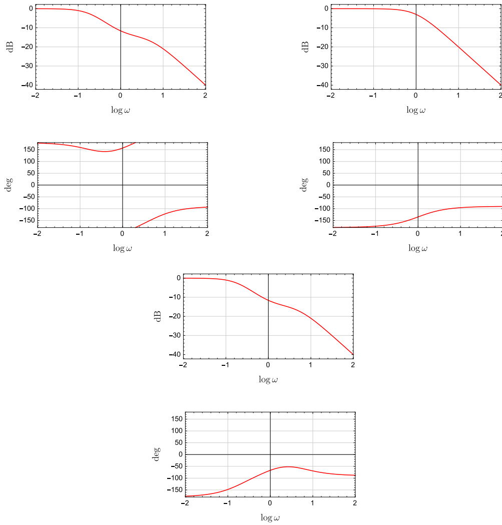
Figure 4.14 Bode plots for (4.4) for \epsilon = -5 , \epsilon = 0 , and \epsilon = 5
