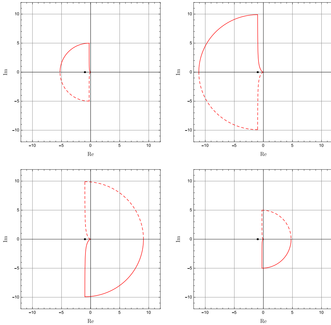
Figure 7.6 The (\infty, 0.1) -Nyquist contours for R_L(s) = \frac{1}{s(s+a)} , a = -2 (top left), a = -1 (top right), a = 1 (bottom left), and a = 2 (bottom right)
