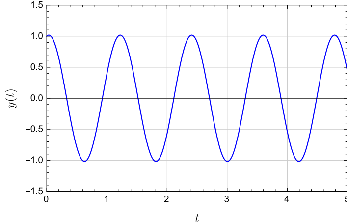
Figure 6.40 Falling mass under proportional control
