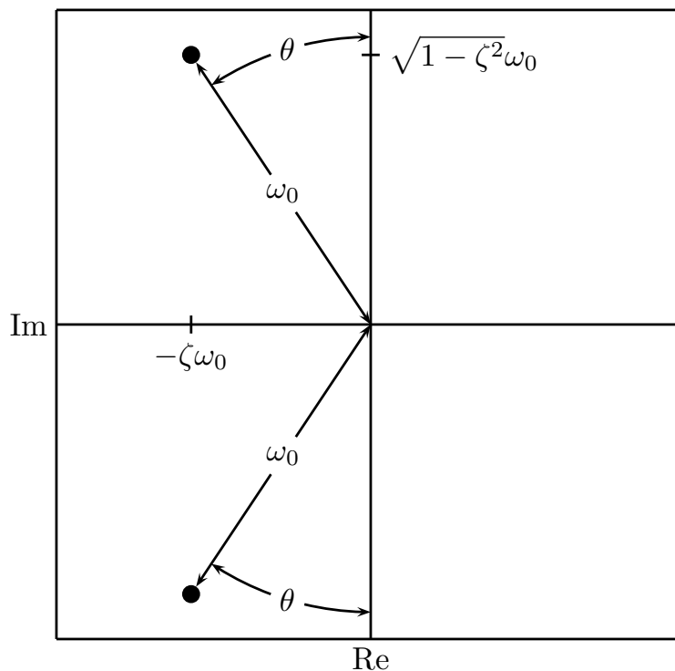
Figure 8.7 Pole locations for T_{\zeta, \omega_0} when 0 < \zeta < 1
