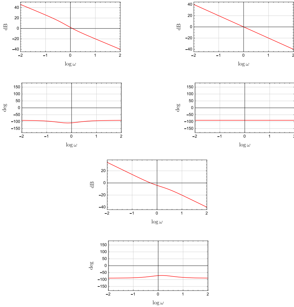
Figure 7.11 Bode plots for R_L(s) = \frac{s+1}{s(s+a)} for a = \frac{1}{2} (top left), a = 1 (top right), and a = 2 (bottom)
