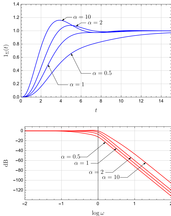
Figure 8.11 The effect of an added pole for \alpha = \frac{1}{2}, 1, 2, 10
