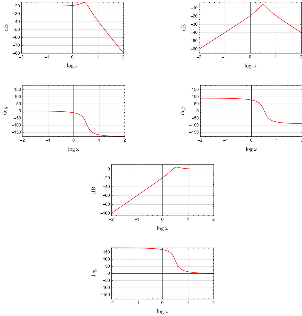
Figure 4.4 The displacement (top left), velocity (top right), and acceleration (bottom) frequency response for the mass-spring damper system when d = 2 and k = 10
