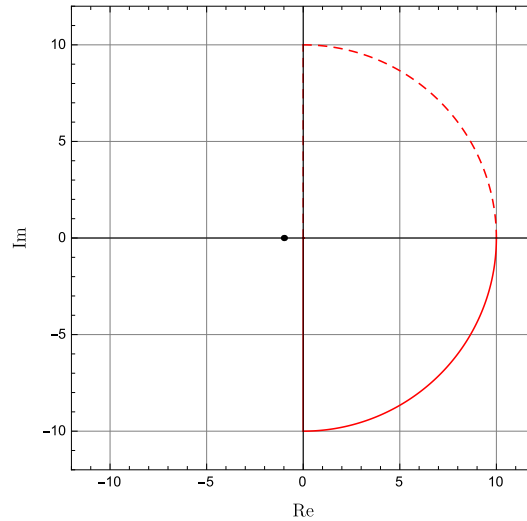
Figure 7.5 The (\infty, 0.1) -Nyquist contour for R_L(s) = \frac{1}{s}
