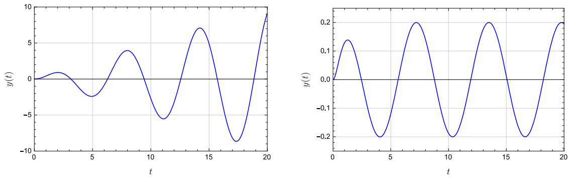
Figure 6.29 Output response for open-loop system (left) and closed-loop system (right) under static state feedback
