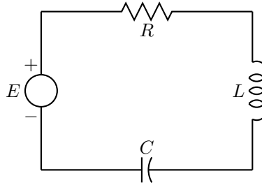
Figure 1.14 A series RLC circuit
