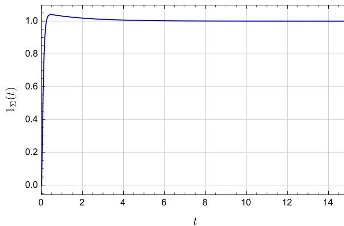
Figure 12.11 Step response of mass with lead compensator
