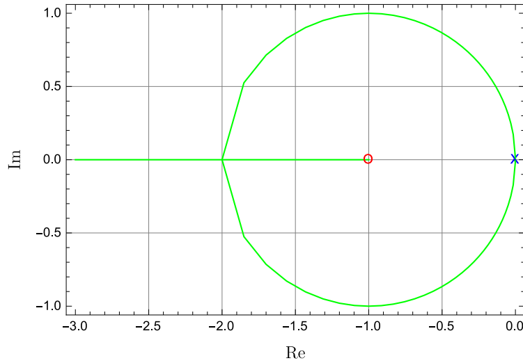
Figure 11.4 Root locus for (N(s), D(s)) = (s + 1, s^2)
