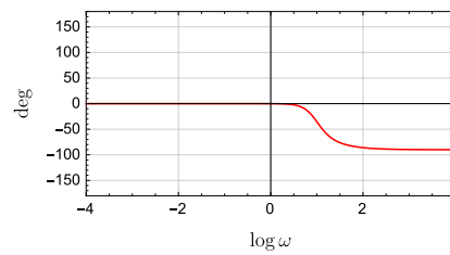
Bode plot 2
