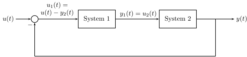
Figure E2.3 SISO linear systems connected in a negative feedback loop
