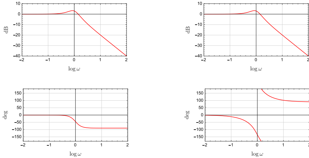
Figure 4.15 Bode plots for the two systems of (4.5) and (4.6)— H_{\Sigma_1} is on the left and H_{\Sigma_2} is on the right
