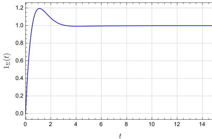
Figure 12.19 Step response of mass with PID controller
