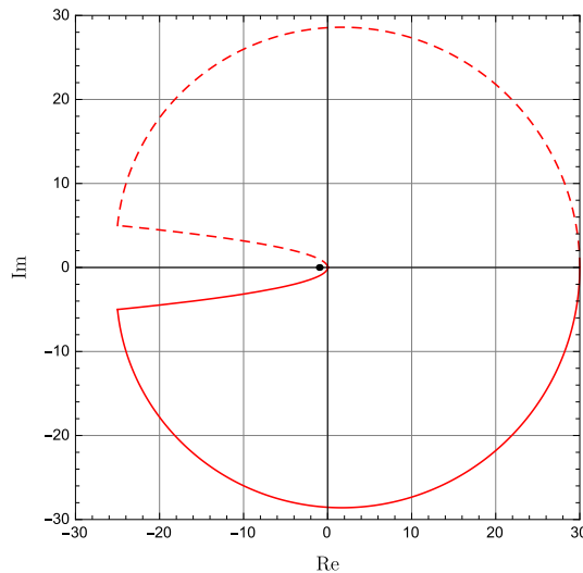
Figure 7.9 The (\infty, 0.2) -Nyquist contour for R_L(s) = \frac{s+1}{s^2}
