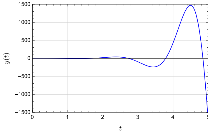
Figure 6.42 Falling mass under integral control
