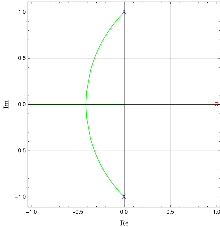
Figure 13.10 Locus of roots for s^2 - Ks + 1 + K where K \in (-1, 0)
