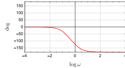
Bode plot 2
