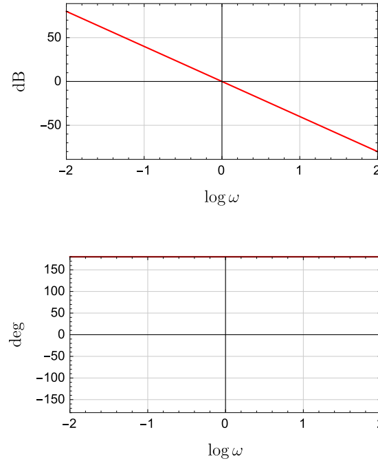
Figure 12.15 Plant Bode plot for mass system
