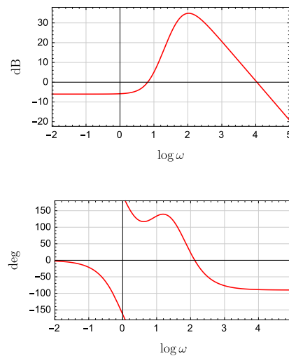
Figure 7.16 Bode plot for BIBO stable transfer function with positive phase margins
