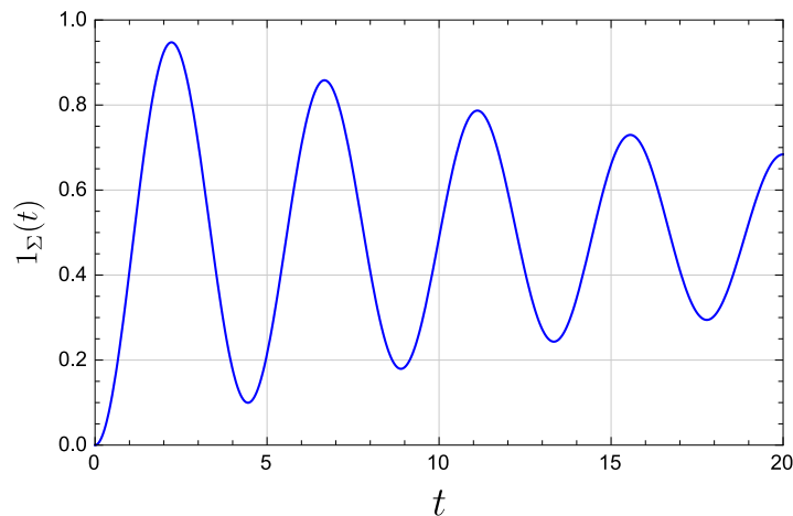
Figure 13.2 Step response for rotor on shaft
