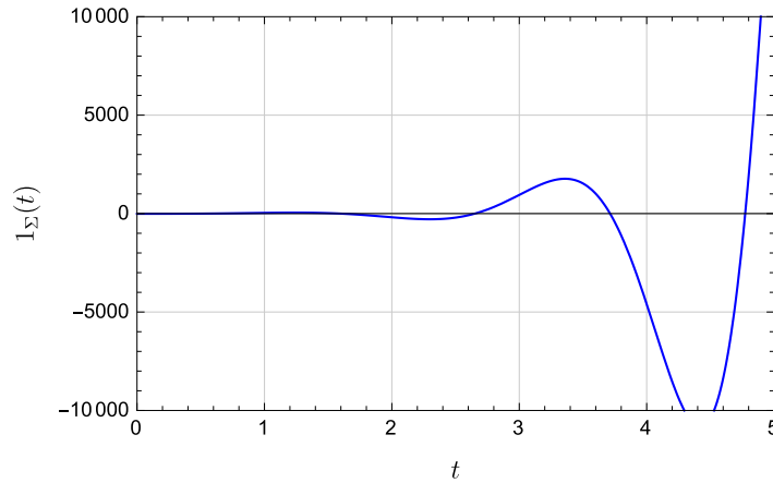
Figure 8.22 Response of falling mass to step disturbance with integral control
