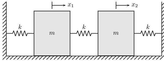
Figure E1.2 Coupled masses
