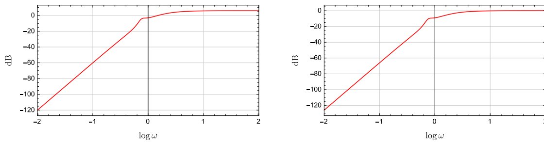
Figure 7.26 The magnitude Bode plot for W_u R_C \bar{S}_L when a = 1 (left) and when a = \frac{1}{2} (right)
