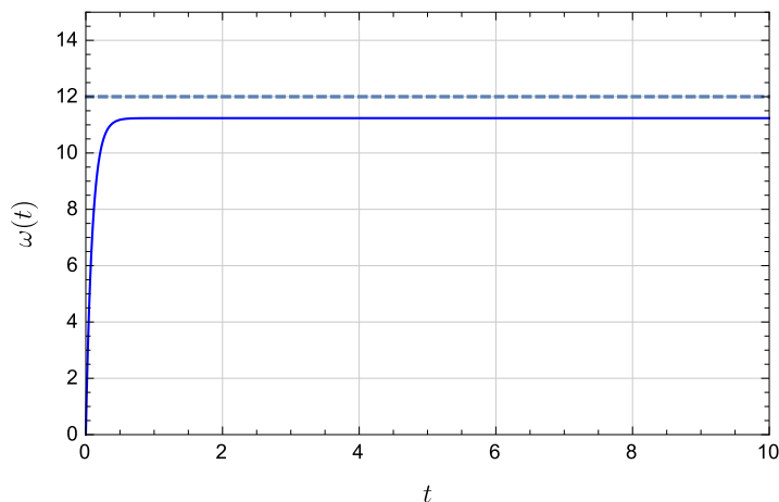
Figure 1.8 Closed-loop response of DC motor with disturbance
