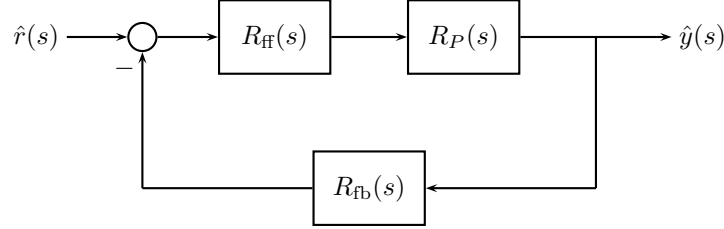
Figure 13.14 A two controller feedback loop
