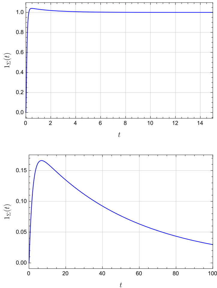
Figure 12.14 Step response of mass (top) and response to step disturbance (bottom) with lead and integrator compensation
