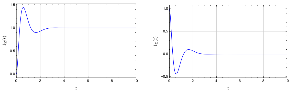
Figure 13.13 Step response (top) and response to step disturbance (bottom)
