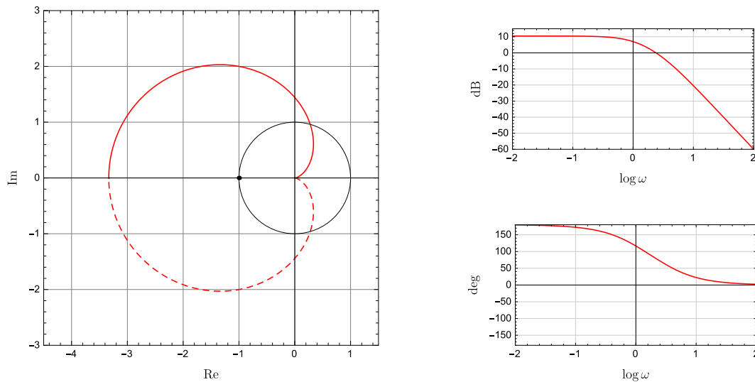
Figure 7.15 Nyquist and Bode plots for R_L(s) = -\frac{10}{s^2 + 4s + 3}
