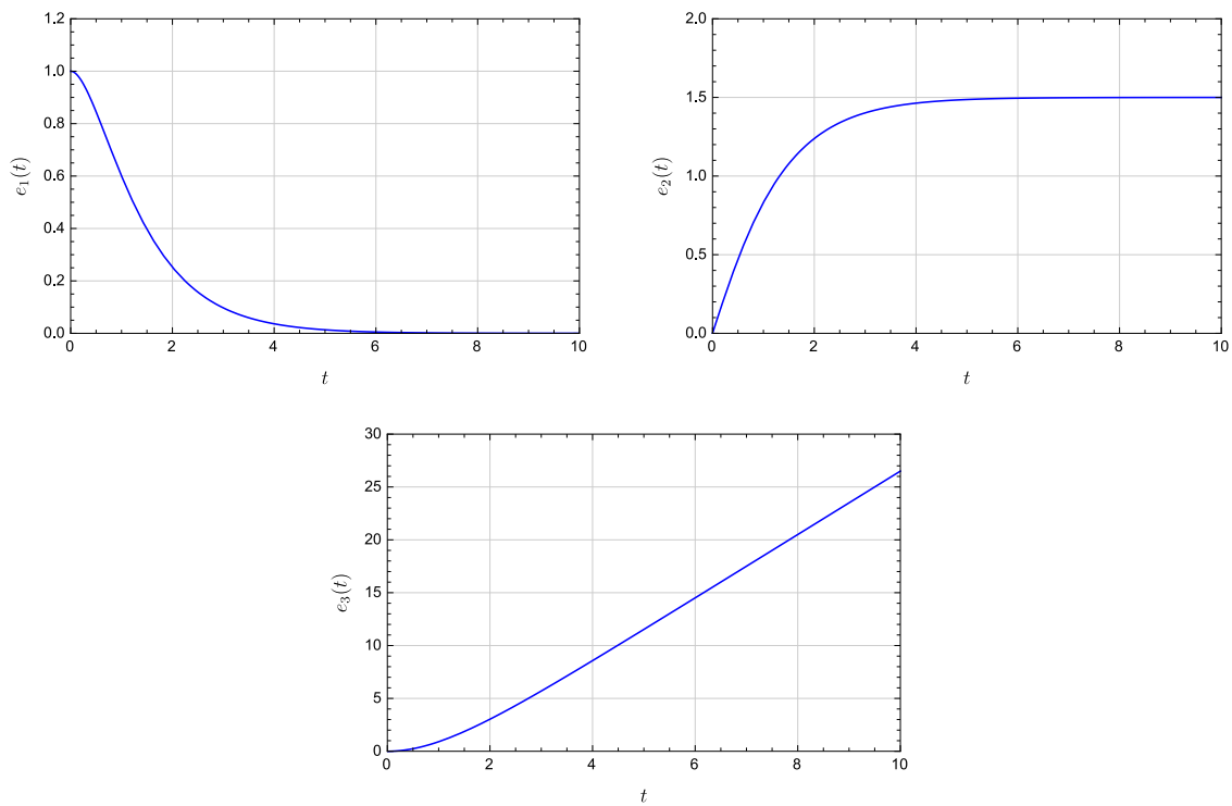
Figure 8.13 Step (top left), ramp (top right), and parabolic (bottom) responses for a system of type 1
