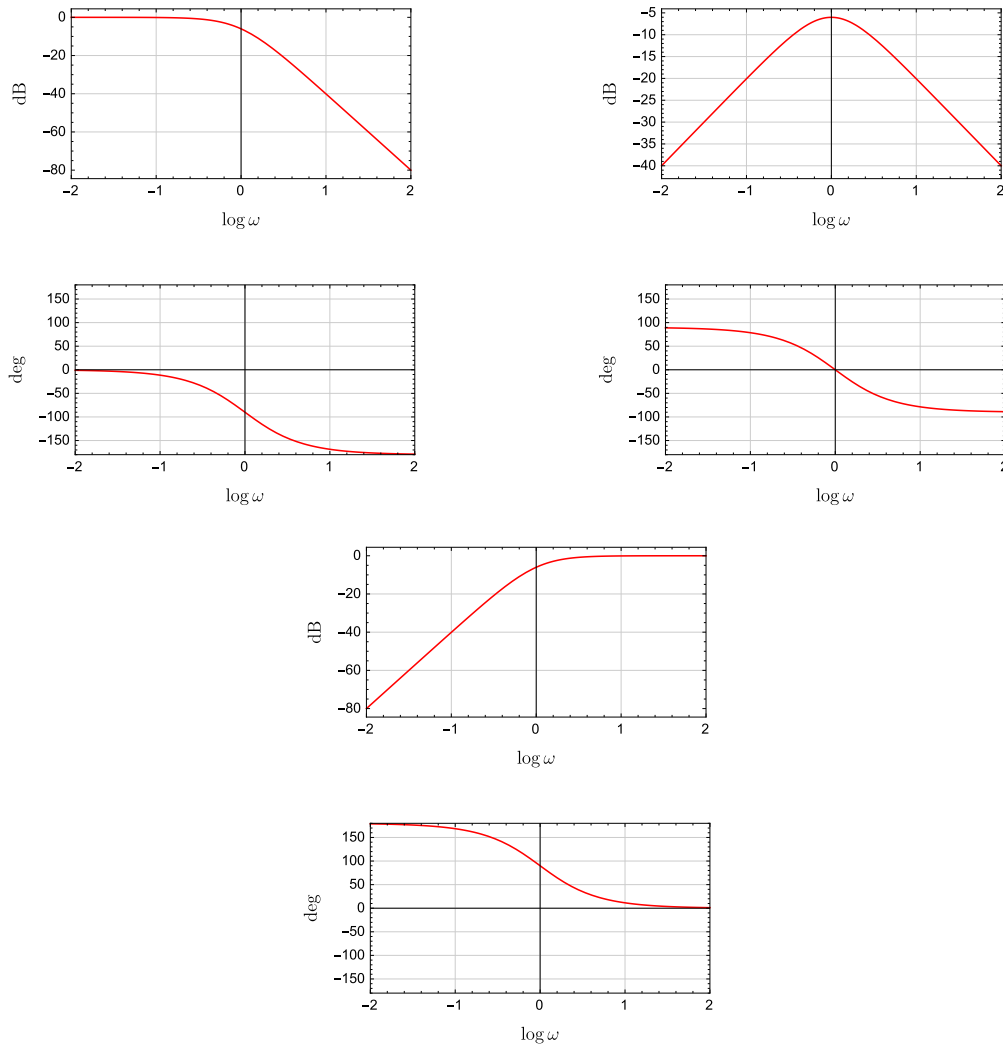
Figure 4.3 The displacement (top left), velocity (top right), and acceleration (bottom) frequency response for the mass-spring damper system when d = 2 and k = 1
