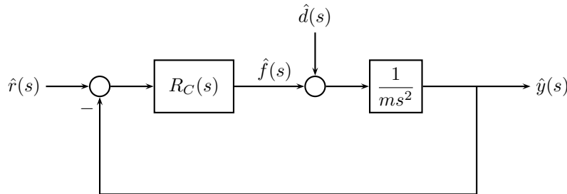
Figure 12.7 Block diagram for controller design for mass
