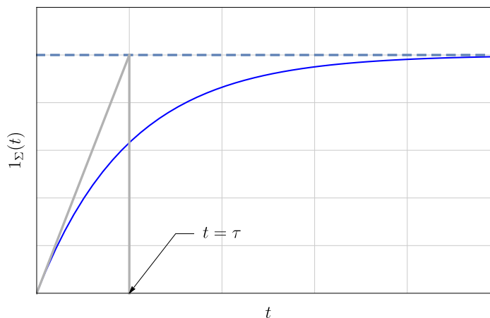
Figure 8.2 Step-response for typical first-order system
