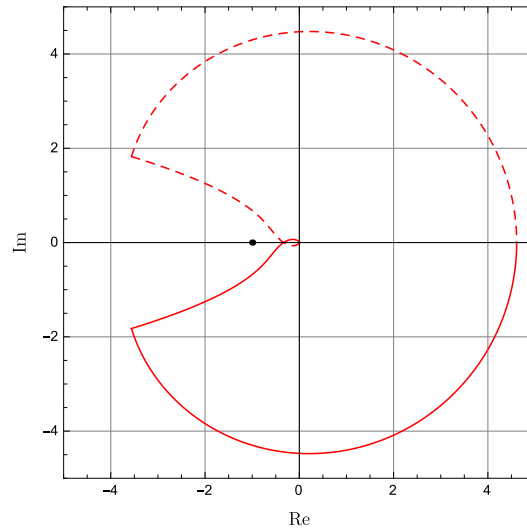
Figure 10.3 Nyquist plot for dynamic output feedback problem
