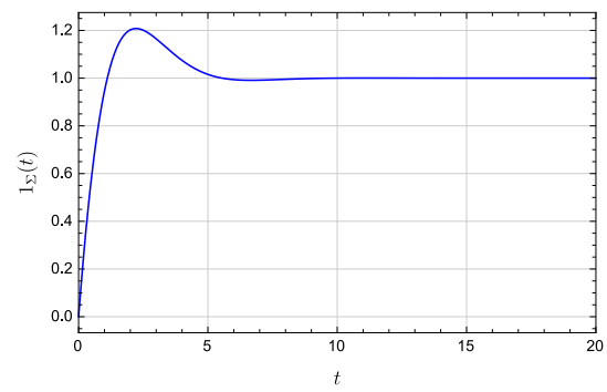
Step response 2
