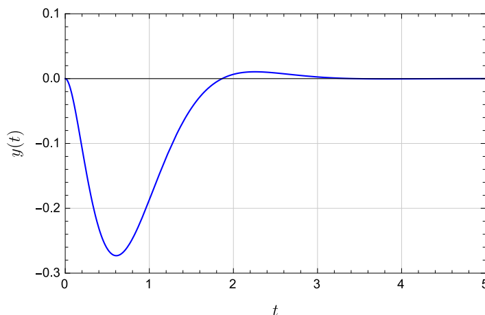
Figure 8.24 Response of falling mass with PID controller
