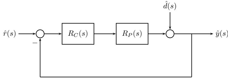
Figure E8.4 Adding a disturbance
