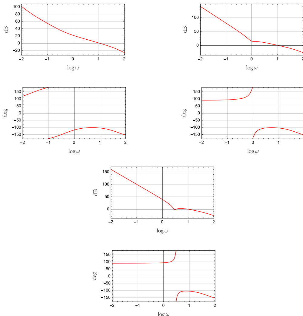
Figure 12.13 Bode plots for mass with lead and integrator compensation: K_I = \frac{1}{10} (top left), K_I = 10 (top right), and K_I = 100 (bottom)
