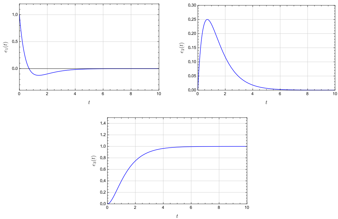
Figure 8.14 Step (top left), ramp (top right), and parabolic (bottom) responses for a system of type 2
