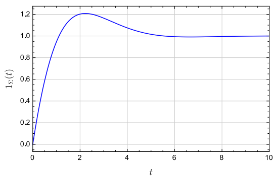
Step response 1
