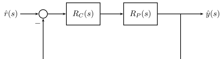
Figure 12.6 Closed-loop system for loop shaping
