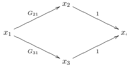
Figure 6.5 The signal flow graph for a parallel interconnection
