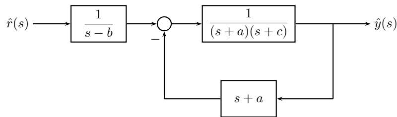
Figure E6.1 A block diagram for determining IBIBO stability
