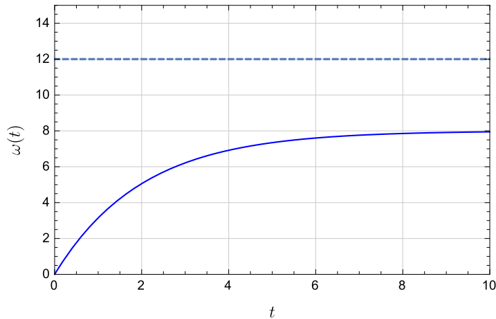
Figure 1.4 Open-loop response of DC motor with disturbance
