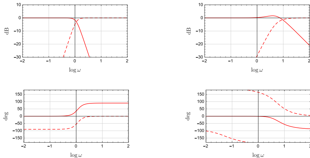
Figure 8.27 Bode plots for the closed-loop transfer function and sensitivity function for the falling mass with integral controller (left) and PID controller (right). In each case, the solid line represents the closed-loop transfer function and the dashed line the sensitivity function.
