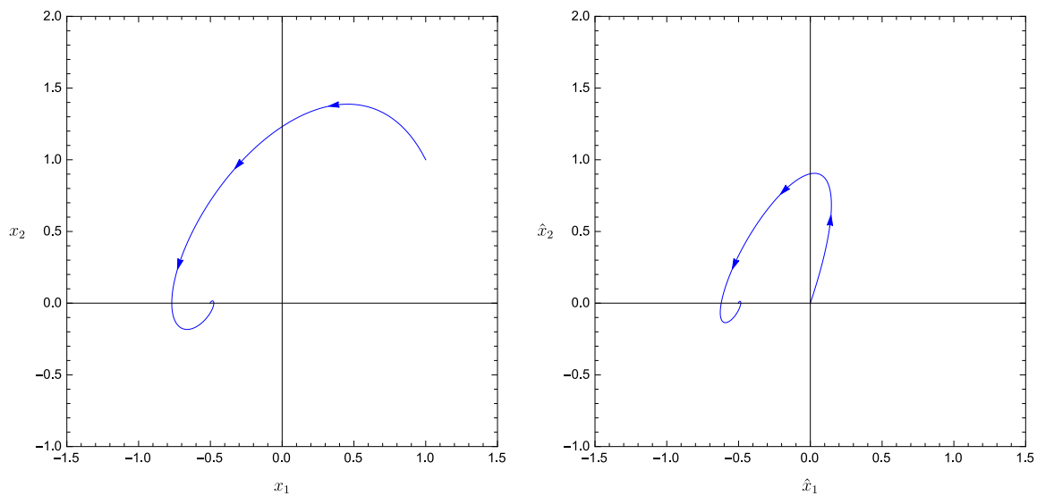
Figure 10.10 The state (left) and the estimated state (right) for the closed-loop system
