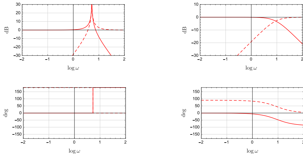
Figure 8.26 Bode plots for the closed-loop transfer function and sensitivity function for the falling mass with proportional controller (left) and derivative controller (right). In each case, the solid line represents the closed-loop transfer function and the dashed line the sensitivity function.
