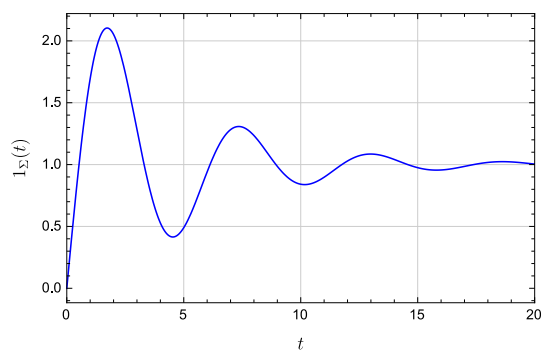
Step response 1
