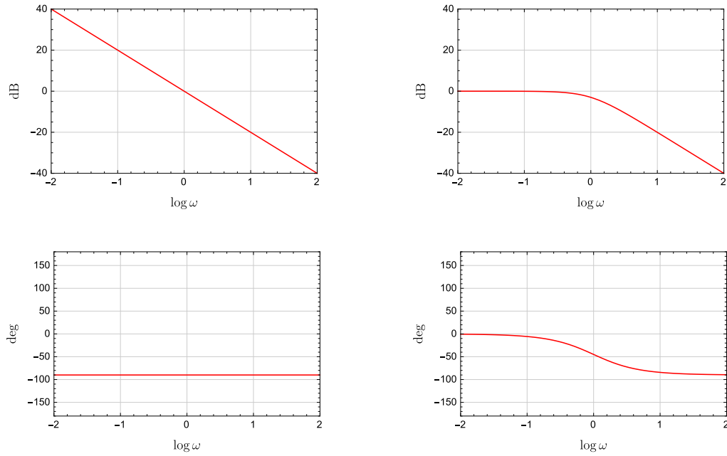
Figure 4.7 Bode plot for H(\omega) = (i\omega)^{-1} (left) and for H(\omega) = (1 + i\omega)^{-1} (right)
