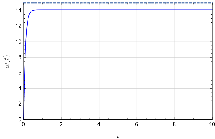
Figure 1.9 Closed-loop response of DC motor with “actual” motor time-constant
