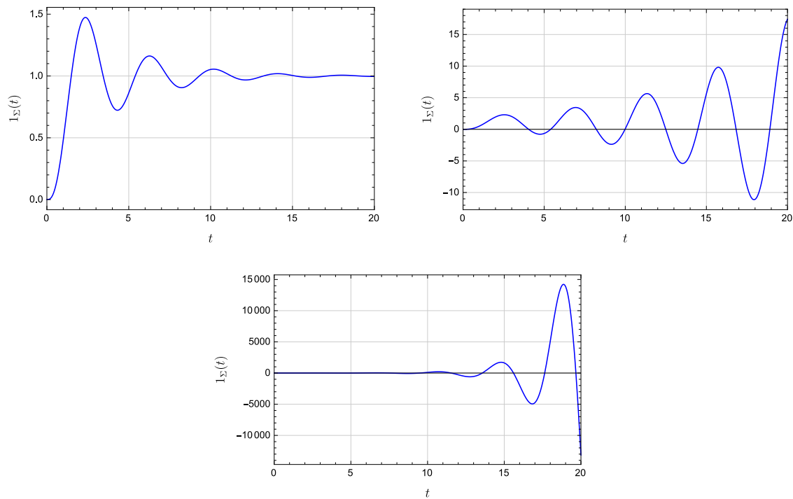
Figure 13.7 Normalised step responses for example using second Ziegler-Nicols tuning method: P (top left), PI (top right), and PID (bottom)
