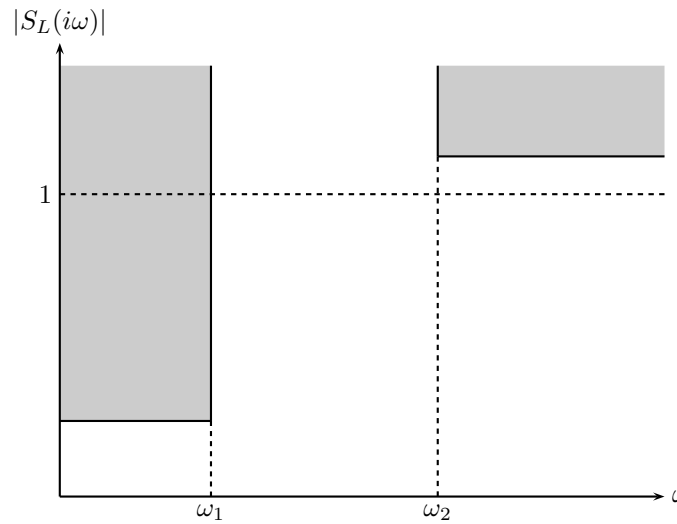
Figure 9.6 Combined sensitivity and complementary sensitivity function restrictions
