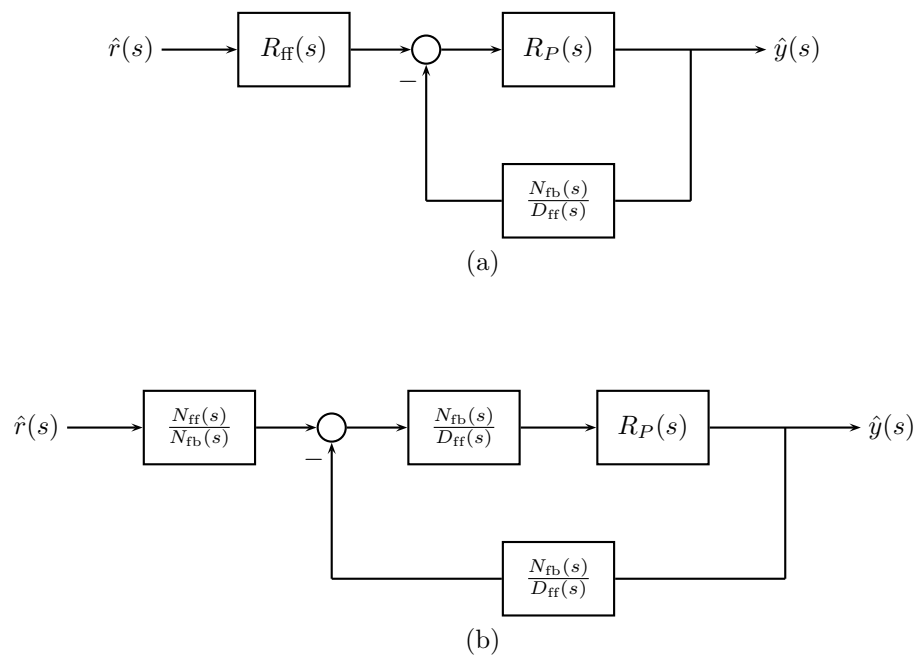
Figure E13.1 Alternate two controller configuration implementations
