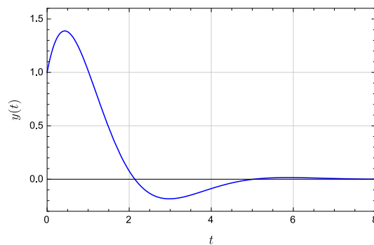
Figure 10.11 The output for the interconnection of Figure 10.8
