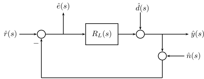
Figure 8.25 Block diagram for investigating the sensitivity function
