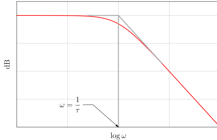
Figure 8.3 Bode plot for typical first-order system
