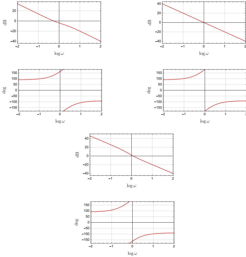
Figure 7.10 Bode plots for R_L(s) = \frac{s+1}{s(s+a)} for a = -2 (top left), a = -1 (top right), and a = -\frac{1}{2} (bottom)
