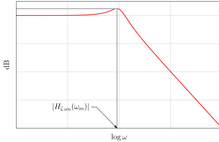
Figure 8.8 Typical Bode plot for second-order system with \zeta < \frac{1}{\sqrt{2}}
