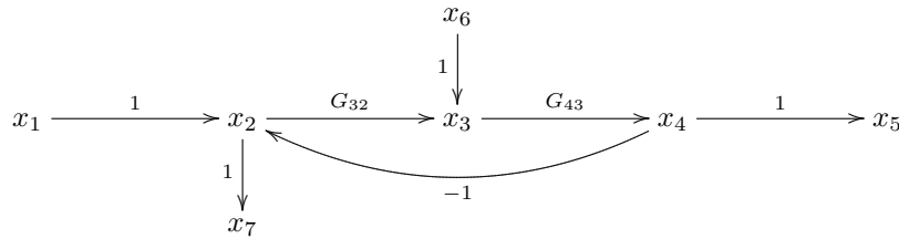
Figure 6.7 Signal flow graph for negative feedback loop with extra structure
