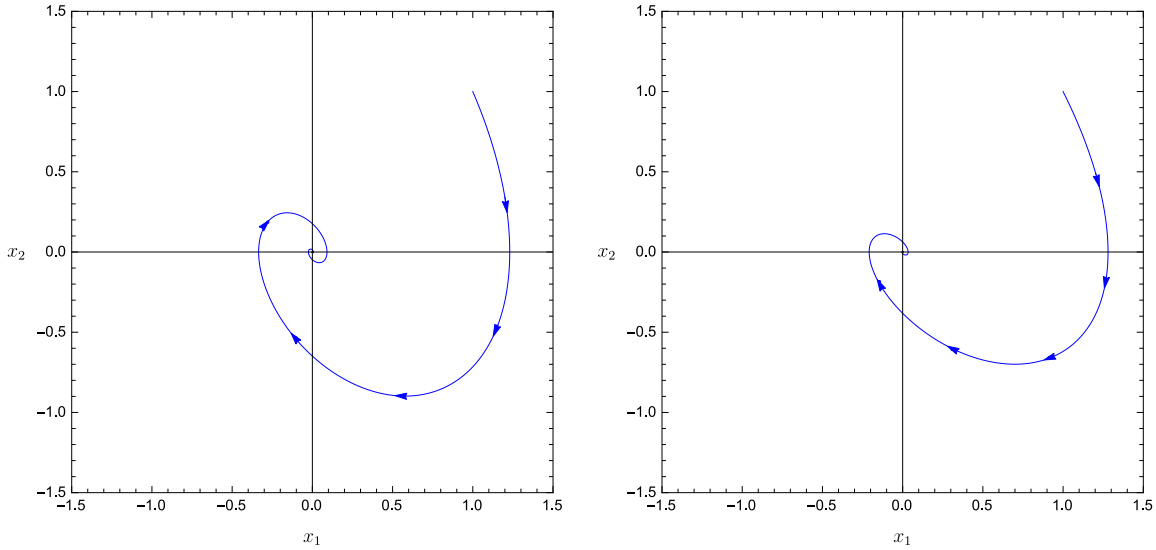
Figure 14.1 Optimal trajectories for output vector \mathbf{c}_1 (left) and \mathbf{c}_2 (right)
