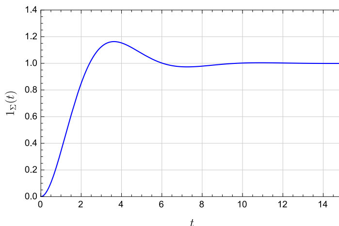
Figure 6.24 Closed-loop step response for simple plant and controller
