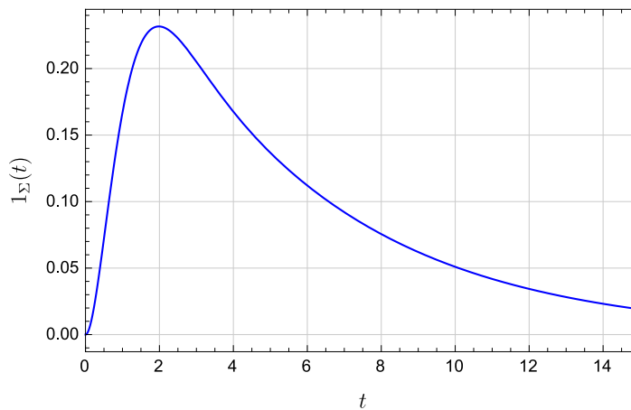
Figure 12.20 Unit step disturbance of mass with PID controller
