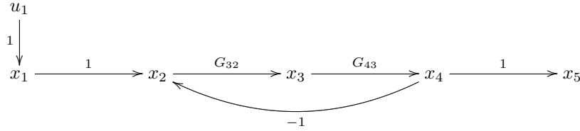
Figure 6.11 Negative feedback signal flow graph with input added
