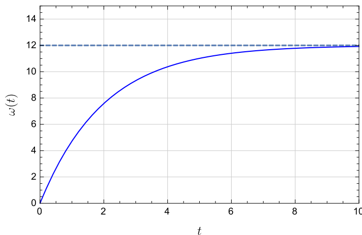
Figure 1.3 Open-loop response of DC motor
