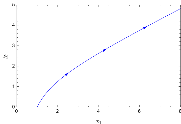
Figure 2.8 The state-space behaviour of (2.7) with a step input and non-zero initial condition
