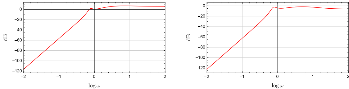
Figure 9.11 Bode plot of |W_u R_C \bar{S}_L| + |W_p \bar{S}_L| for a = 1 (left) and for a = \frac{1}{4} (right)
