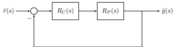
Figure 7.2 A unity feedback loop
