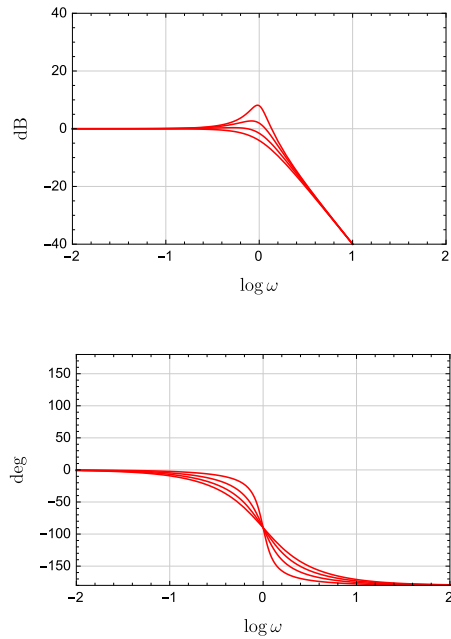
Figure 4.8 Bode plot for H(\omega) = (1 + 2i\zeta\omega - \omega^2)^{-1} for \zeta = 0.2, 0.4, 0.6, 0.8
