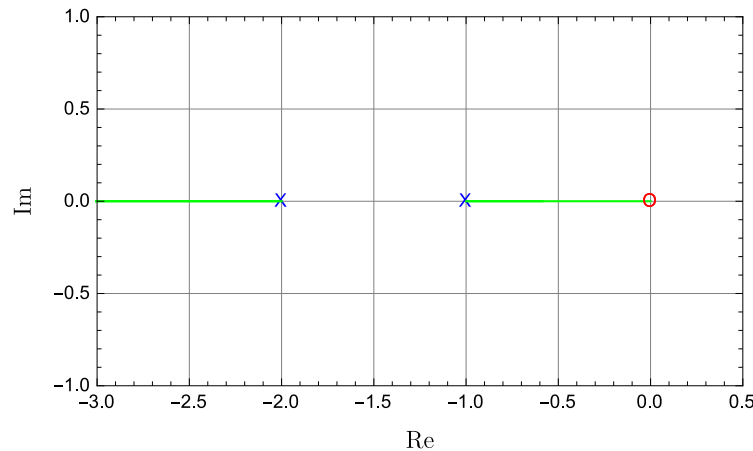
Figure 6.37 The locus of roots for (6.15) with derivative control
