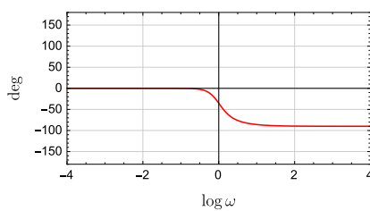
Bode plot 1
