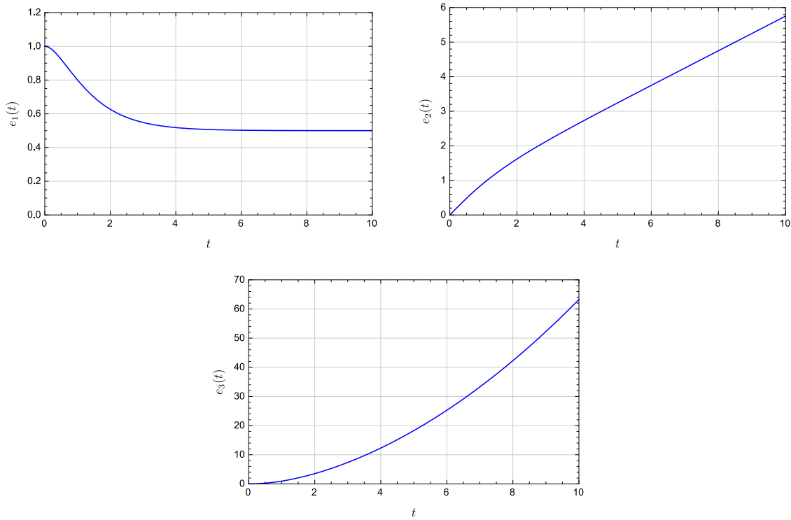
Figure 8.12 Step (top left), ramp (top right), and parabolic (bottom) error responses for a system of type 0
