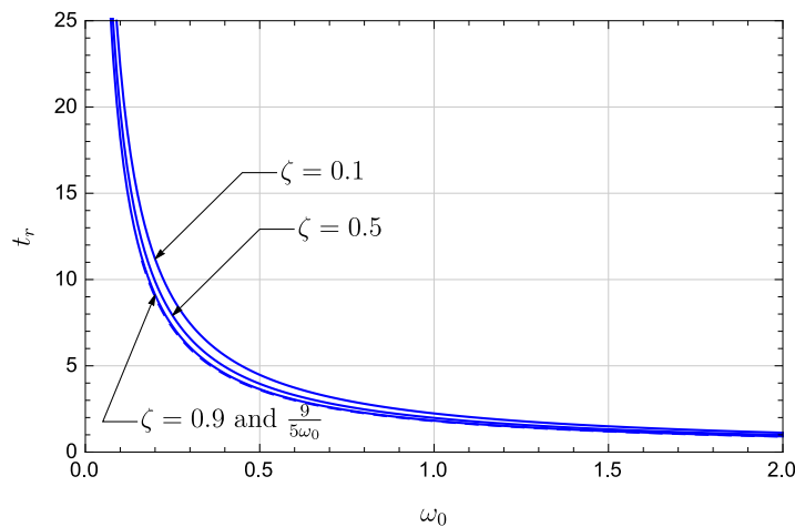
Figure 8.6 Behaviour of rise time versus \omega_0 for various \zeta < 1
