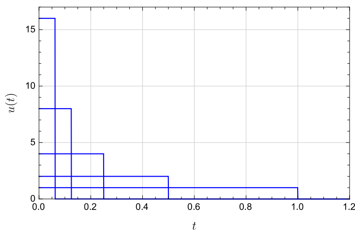
Figure 2.15 A sequence of inputs giving the impulse response in the limit
