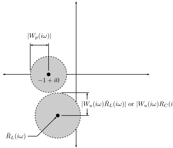
Figure 9.9 Graphical interpretation of robust performance condition
