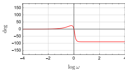
Bode plot 1
