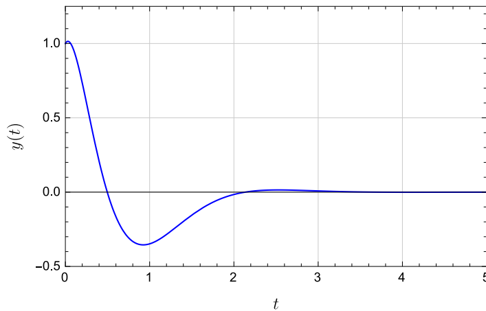
Figure 6.43 Falling mass under combined PID control
