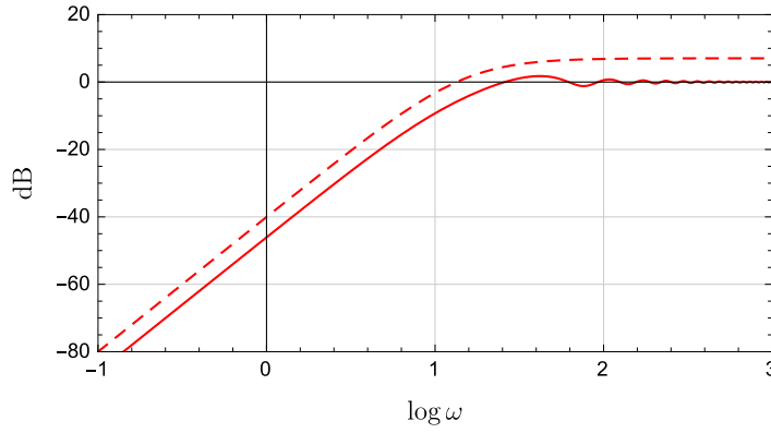
Figure 4.18 \left| \frac{e^{-i\omega/10}}{1-s/10} - 1 \right| (solid) and W_u = \frac{1}{1-\omega^2/15} (dashed)
