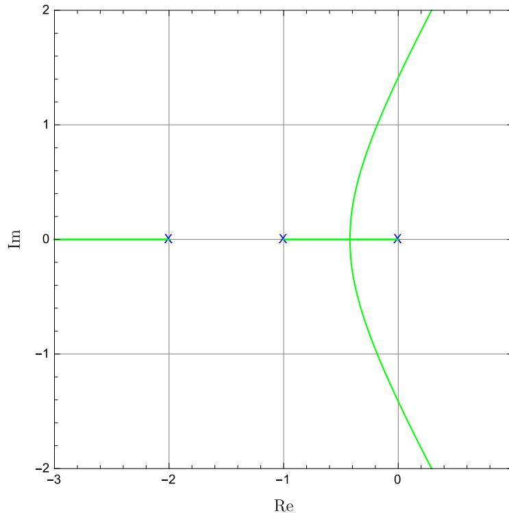
Figure 6.38 The locus of roots for (6.15) with integral control
