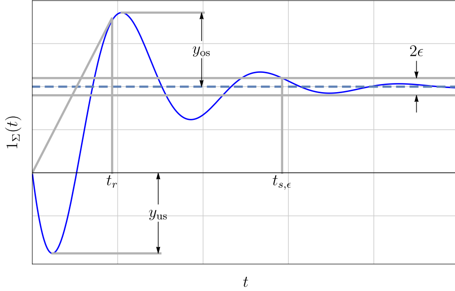
Figure 8.1 Performance parameters in the time-domain
