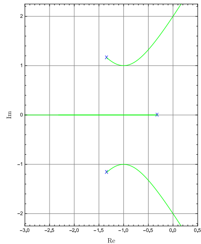
Figure 13.5 Behaviour of poles for plant R_P(s) = \frac{1}{s^3+3s^2+4s+1} and R_C(s) = K as K varies
