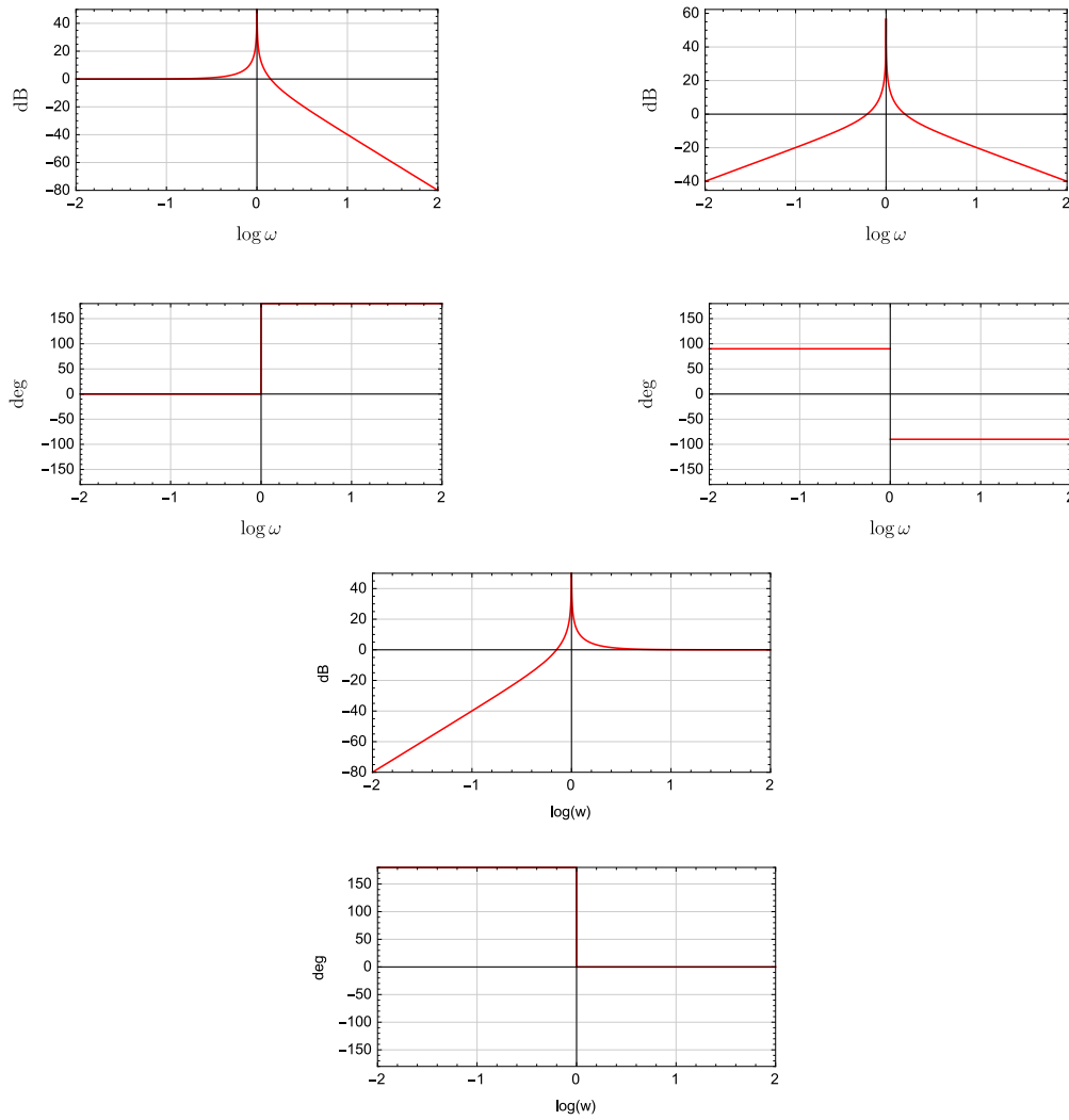
Figure 4.5 The displacement (top left), velocity (top right), and acceleration (bottom) frequency response for the mass-spring damper system when d = 0 and k = 1
