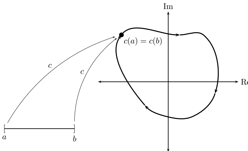
Figure D.2 A closed curve in \mathbb{C}
