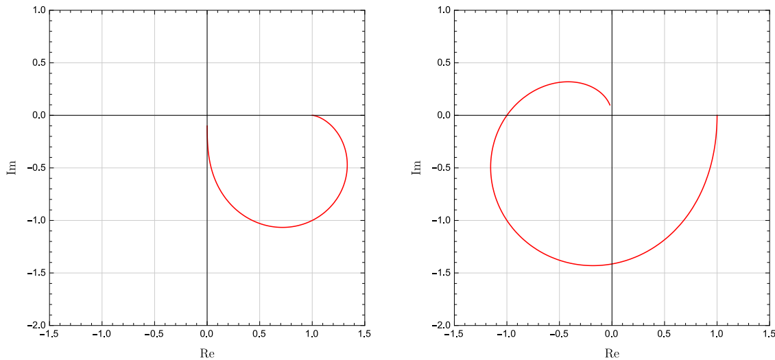
Figure 4.13 Polar plots for minimum phase (left) and nonminimum phase (right) systems
