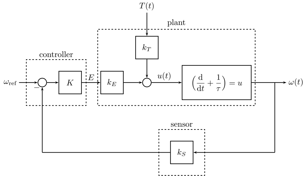
Figure 1.6 DC motor closed-loop control schematic
