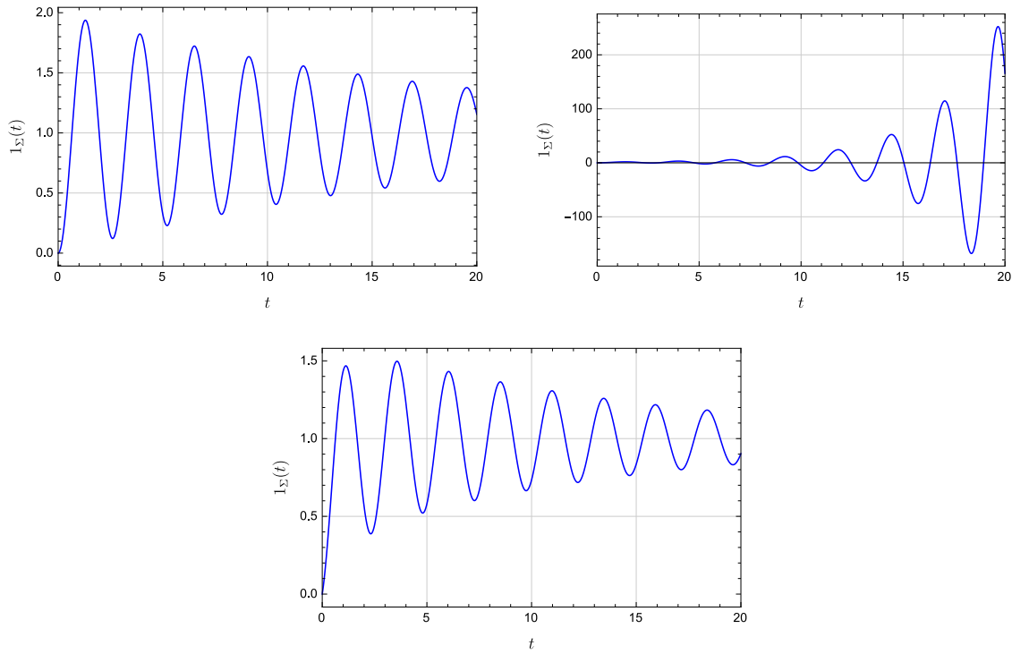
Figure 13.3 Normalised step responses for rotor example using first Ziegler-Nichols tuning method: P (top left), PI (top right), and PID (bottom)
