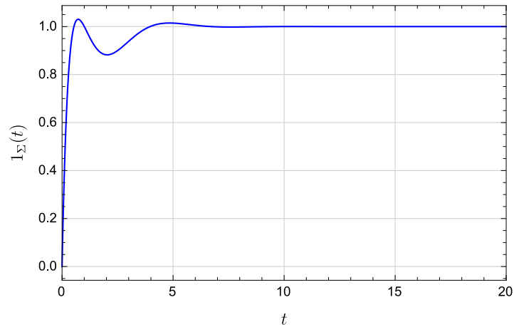
Figure 13.4 Normalised step response for rotor example using first Ziegler-Nicols tuning method and derivative time adjusted to T_D = 1
