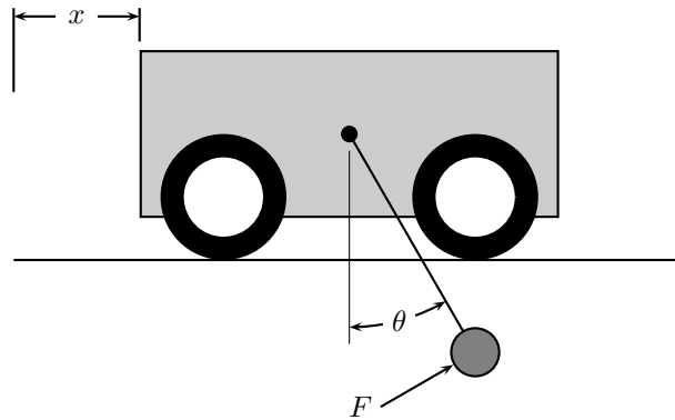
Figure E10.1 The pendulum/cart with an alternate input
