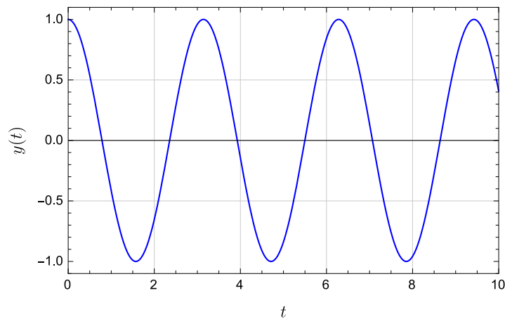
Figure 2.4 Acceleration output for mass-spring system
