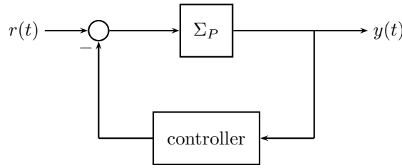
Figure 6.32 A proposed feedback loop for dynamic output feedback
