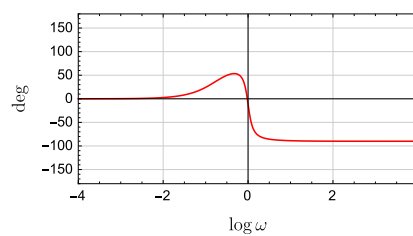
Bode plot 2
