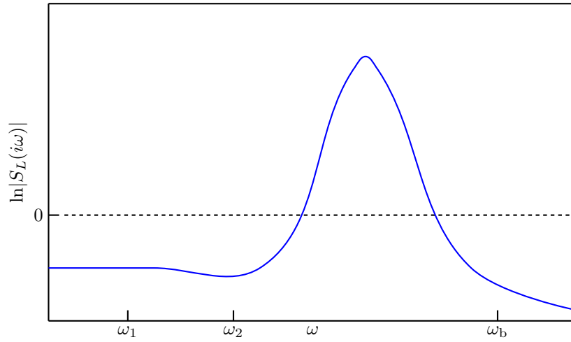
Figure 9.5 The effect of loop gain bandwidth constraints on the sensitivity function area distribution
