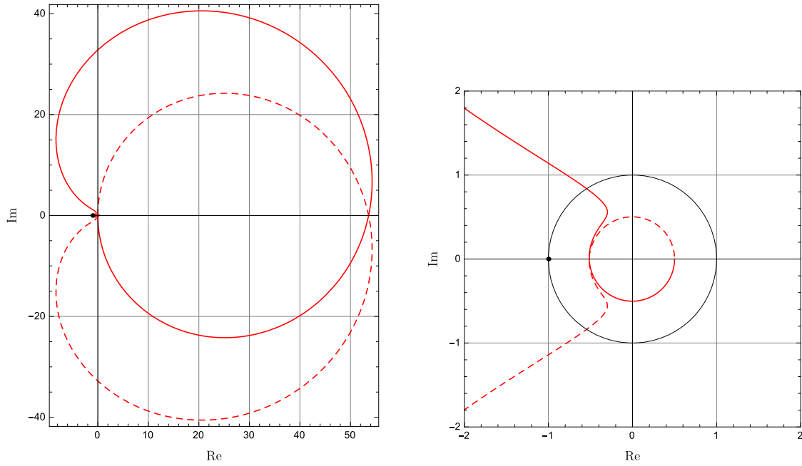
Figure 7.17 Nyquist contour for BIBO stable transfer function with positive phase margins
