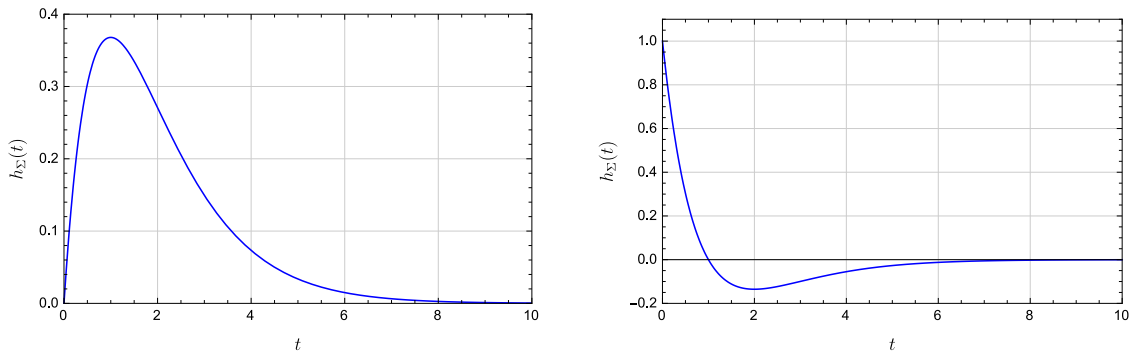
Figure 2.12 The displacement and velocity impulse response for a mass-spring-damper system with m = 1 , d = 2 , and k = 1
