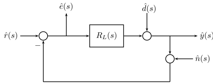
Figure 6.25 A unity gain feedback loop
