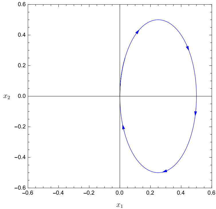
Figure 2.1 Phase curve for step response of mass-spring system
