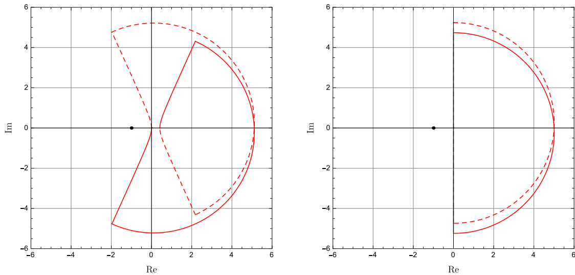
Figure 14.3 Nyquist plots for the optimal state feedback vectors of Example 14.36
