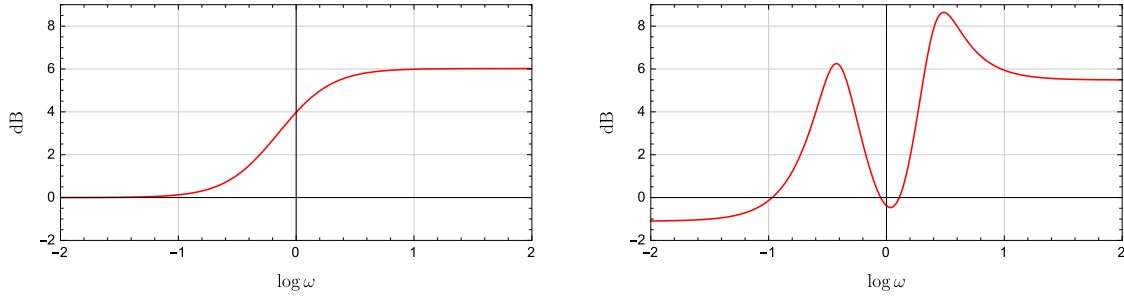
Figure 7.19 Magnitude bode plot for the sensitivity function with loop gain R_{C,1}R_P (left) and R_{C,2}R_P (right)
