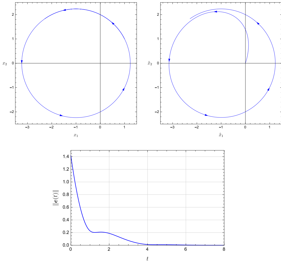
Figure 10.7 The state (top left), the estimated state (top right), and the norm of the error for a Luenberger observer
