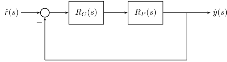
Figure 13.8 Feedback loop for polynomial pole placement
