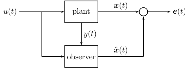
Figure 10.5 A schematic for an observer using the error
