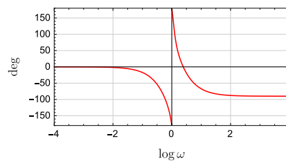
Bode plot 2
