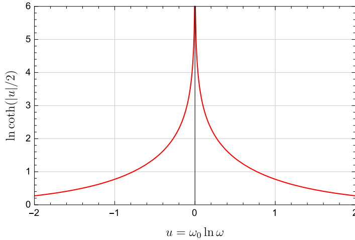
Figure 4.17 The weighting factor in Bode's Gain/Phase Theorem
