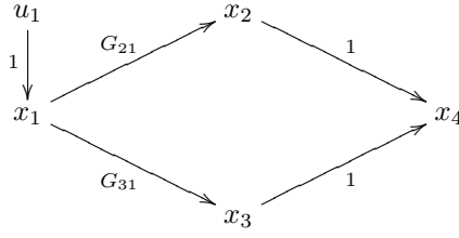
Figure 6.10 Parallel signal flow graph with input added
