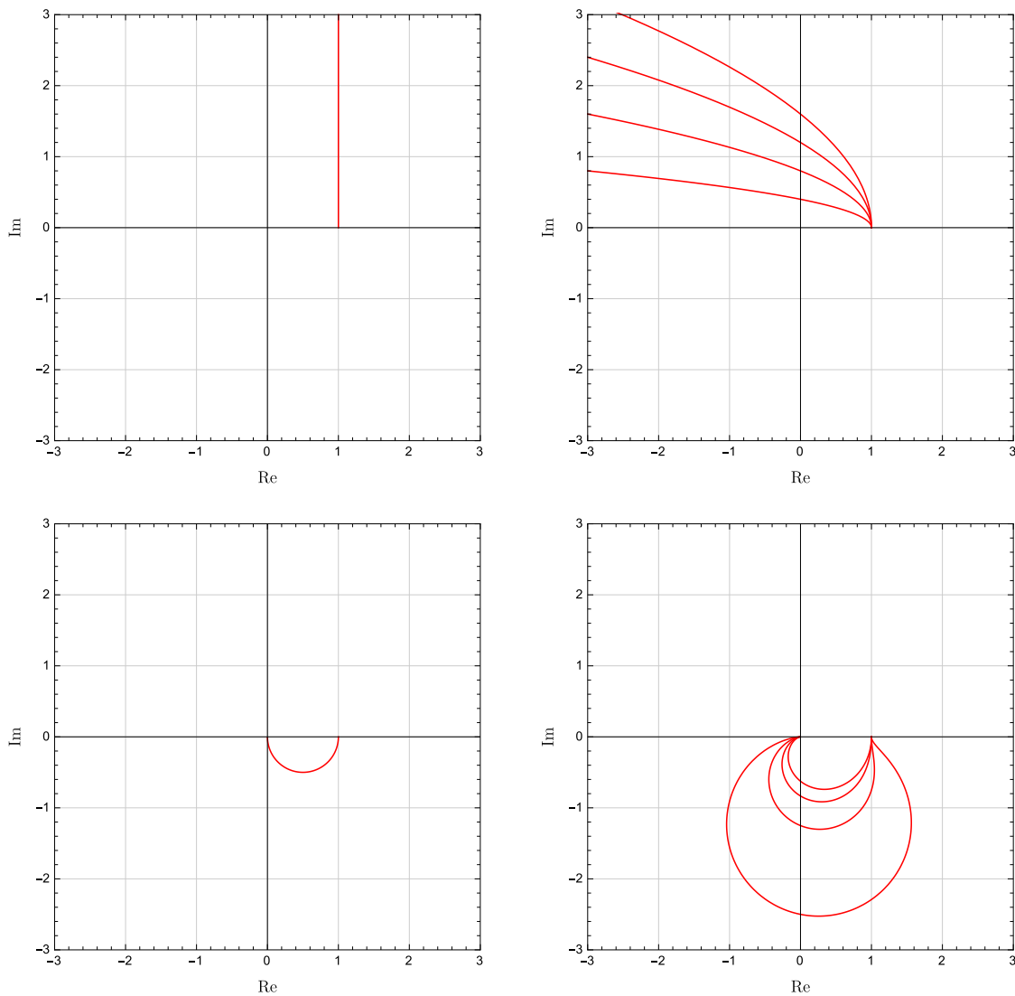
Figure 4.12 Polar plots for H(\omega) = 1 + i\omega (top left), H(\omega) = 1 + 2i\zeta\omega - \omega^2 , \zeta = 0.2, 0.4, 0.6, 0.8 (top right), H(\omega) = (1 + i\omega)^{-1} (bottom left), and H(\omega) = (1 + 2i\zeta\omega - \omega^2)^{-1} , \zeta = 0.2, 0.4, 0.6, 0.8
