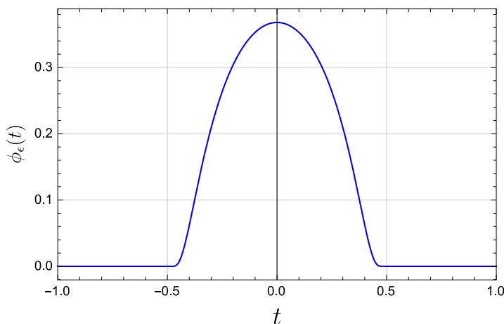
Figure E.1 The test function \phi_\epsilon when \epsilon = 0.5
