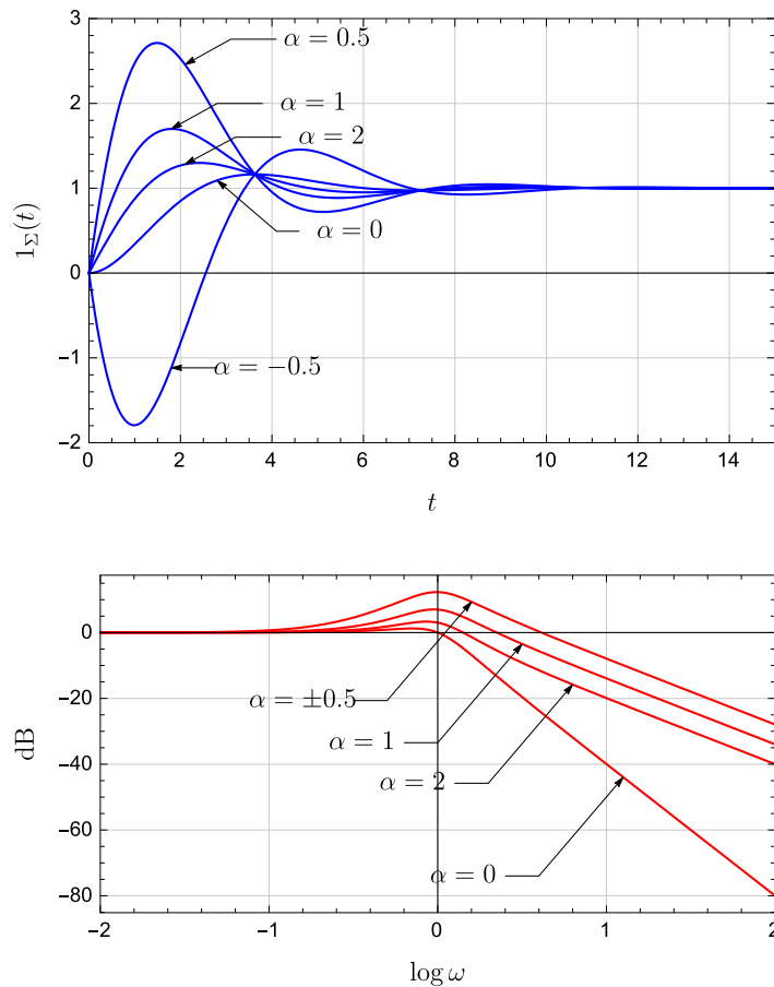
Figure 8.10 The effect of an added zero for \alpha = -\frac{1}{2}, 0, \frac{1}{2}, 1, 2
