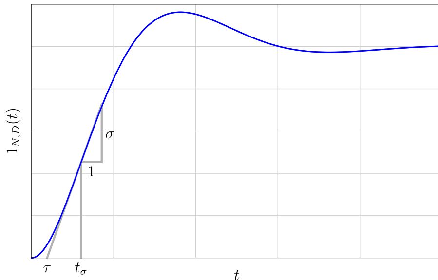
Figure 13.1 The definitions of \sigma and \tau for Ziegler-Nicols PID tuning
