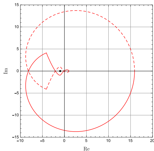
Figure 7.27 Nyquist plot for perturbed plant under additive uncertainty
