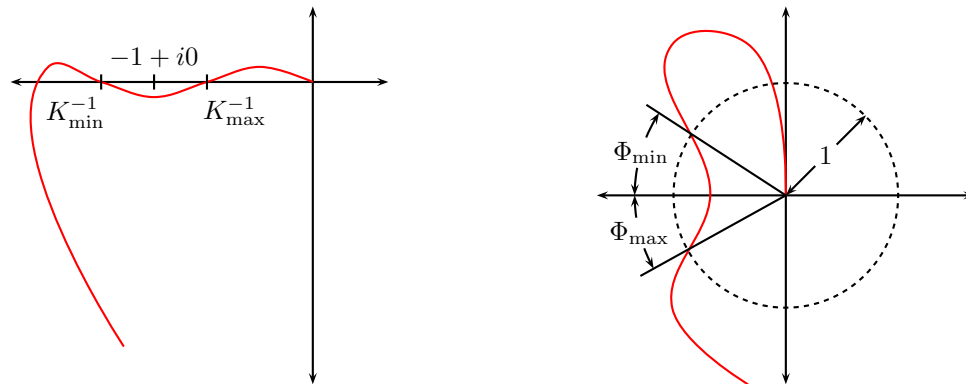
Figure 7.13 Getting gain (left) and phase (right) margins from the Nyquist plot
