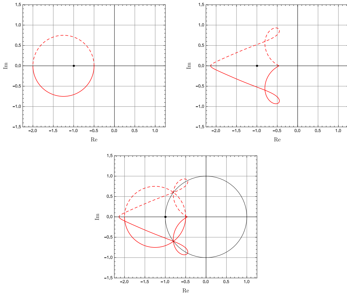
Figure 7.18 Nyquist plots for plant R_P(s) = \frac{2-s}{2s-1} with controller R_{C,1} (top left), with controller R_{C,2} (top right), and both (bottom)
