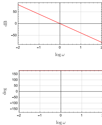
Figure 12.8 Plant Bode plot for mass system
