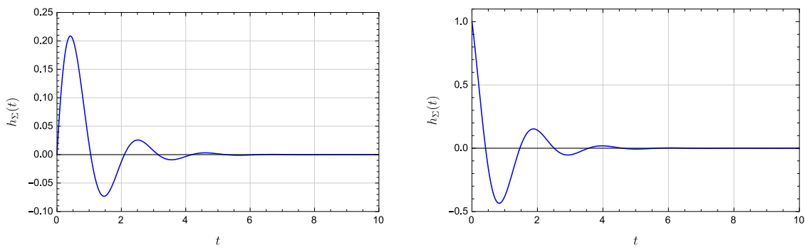
Figure 2.13 The displacement and velocity impulse response for a mass-spring-damper system with m = 1 , d = 2 , and k = 10
