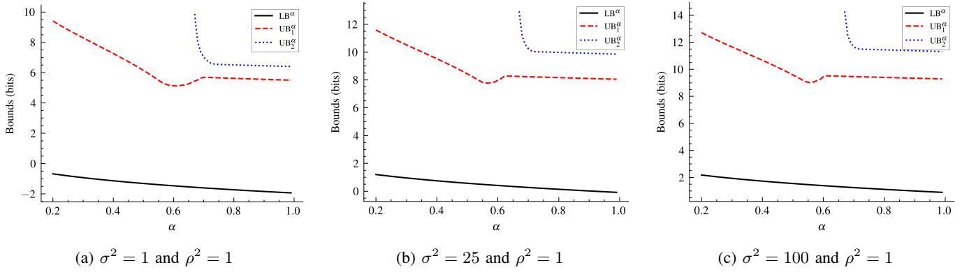
Fig. 2: Comparison of the bounds on the Campbell cost for the AWGN channel, for 0.2 < \alpha < 1 .
