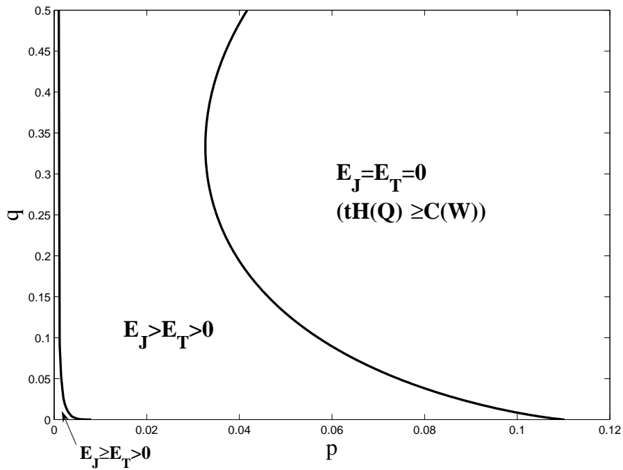
Figure 2: The regions for the ternary SEM source and the binary SEM channel of Example 2 with t = 0.5 .
