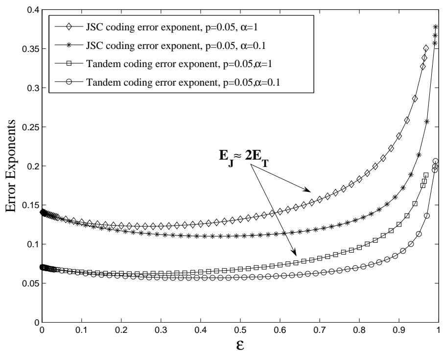
Figure 5: Comparison of E_J and E_T for the SEM source and the QBC of Example 3 with t = 1 .
