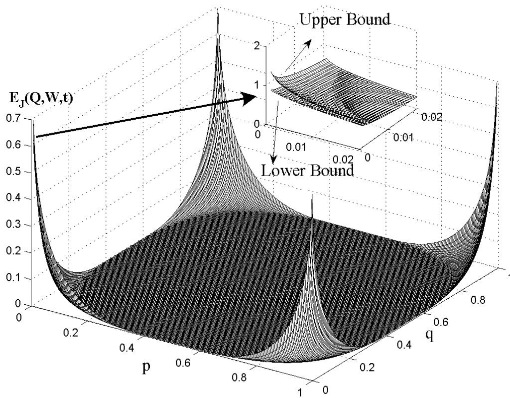
Figure 1: The lower and upper bounds of E_J for the binary SEM source and the binary SEM channel of Example 1 with t = 1 .
