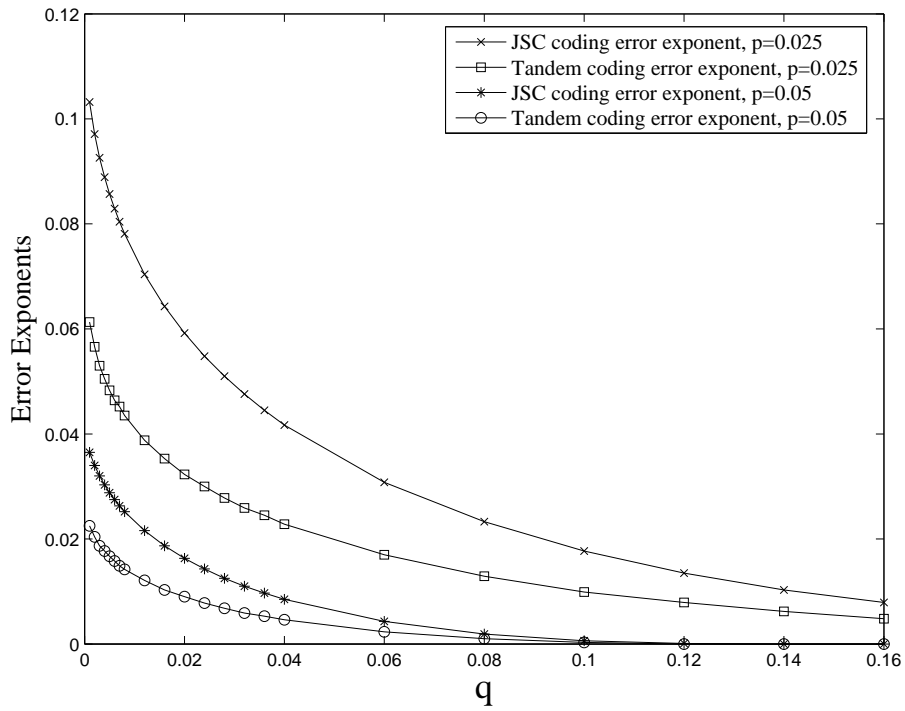
Figure 3: Comparison of E_J and E_T for the ternary SEM source and the binary SEM channel of Example 2 with t = 0.5 .
