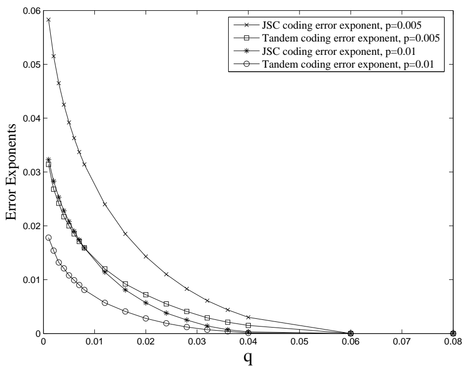
Figure 4: Comparison of E_J and E_T for the ternary SEM source and the binary SEM channel of Example 2 with t = 0.75 .
