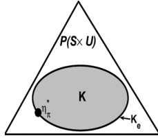
Fig. 2. A schematic representation of the optimization problem (3). The large triangular space is the infinite-dimensional Prohorov space \mathcal{P}(\mathcal{S} \times \mathcal{U}) . Its gray-shaped subset represents the close convex set K of all occupation measures. The set of extreme points of K is K_e and corresponds to the set of all occupation measures associated to stationary deterministic policies. The optimal value of the linear functional \boldsymbol{\eta} \mapsto \langle \boldsymbol{\eta}, g \rangle happens to be achieved on K_e and thus corresponds to the occupation measure \boldsymbol{\eta}^* associated to an optimal deterministic stationary policy \pi^* : \mathcal{S} \rightarrow \mathcal{X} .
